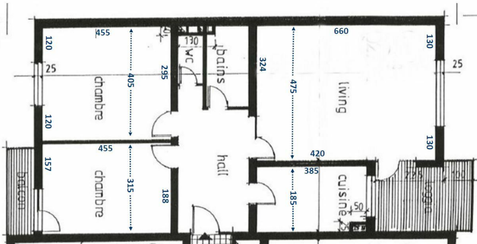
Plan with dimensions
